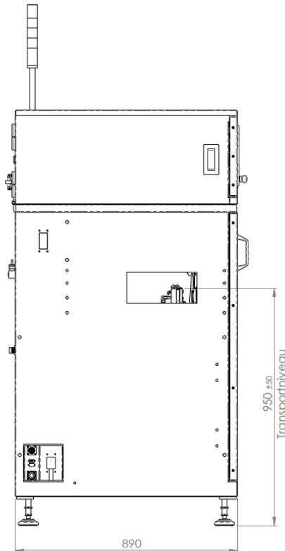
side view
